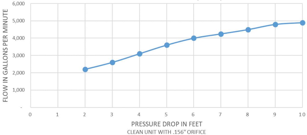
FLOW VS. PRESSURE DROP (FEET)
