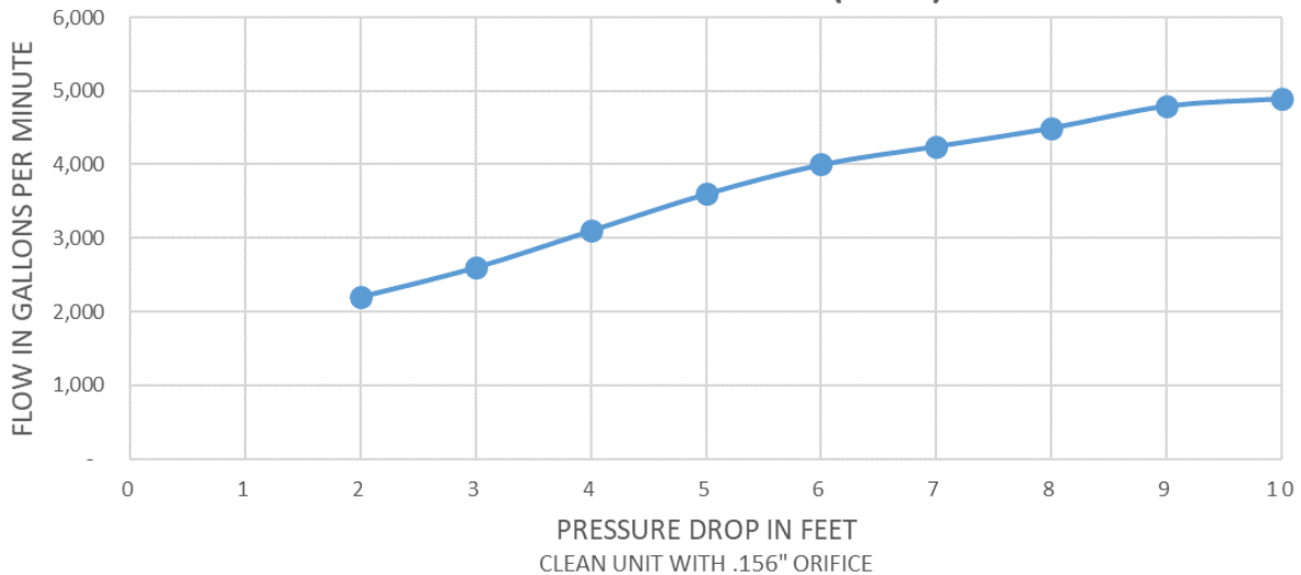
FLOW VS. PRESSURE DROP (FEET)
